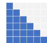
GPT (decoder): sees only the past
