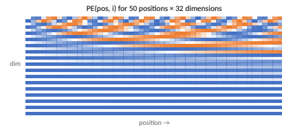
Low dimensions oscillate fast, high dimensions slowly: every position gets a unique pattern.
