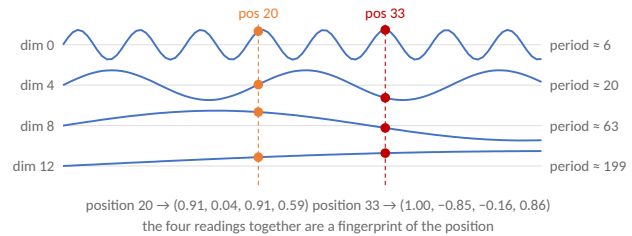
Low dimensions oscillate fast, high dimensions slowly: every position gets a unique pattern.
