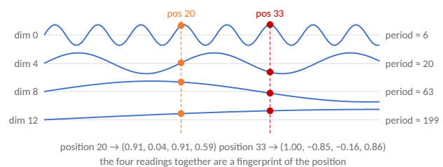
Low dimensions oscillate fast, high dimensions slowly: every position gets a unique pattern.
