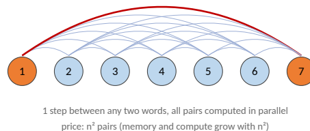
Attention: every pair in one step
