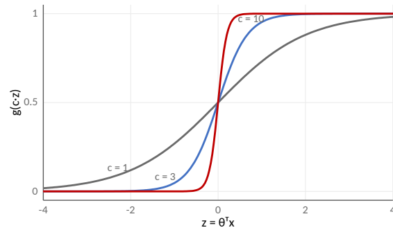
g(cz) for c = 1, 3, 10 : the same boundary, ever more confident.
