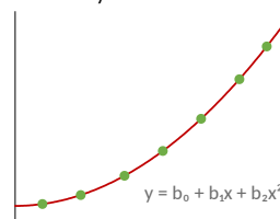
Polynomial model
