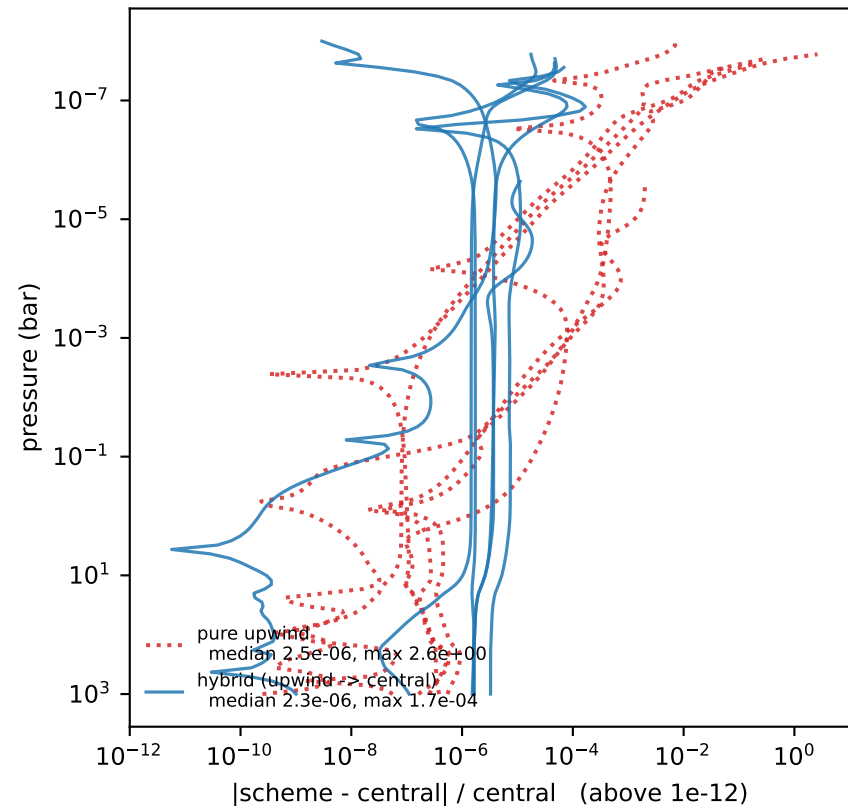
C the hybrid returns the central fixed point
