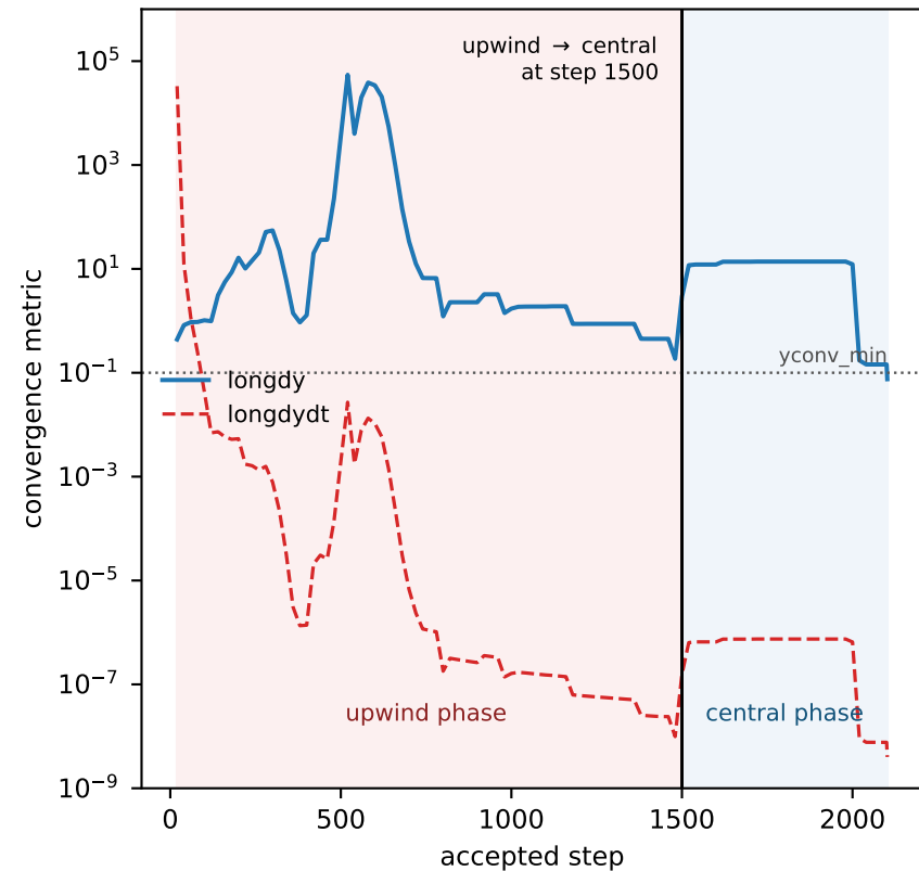
A hybrid run: 'converged' at 2102 steps
