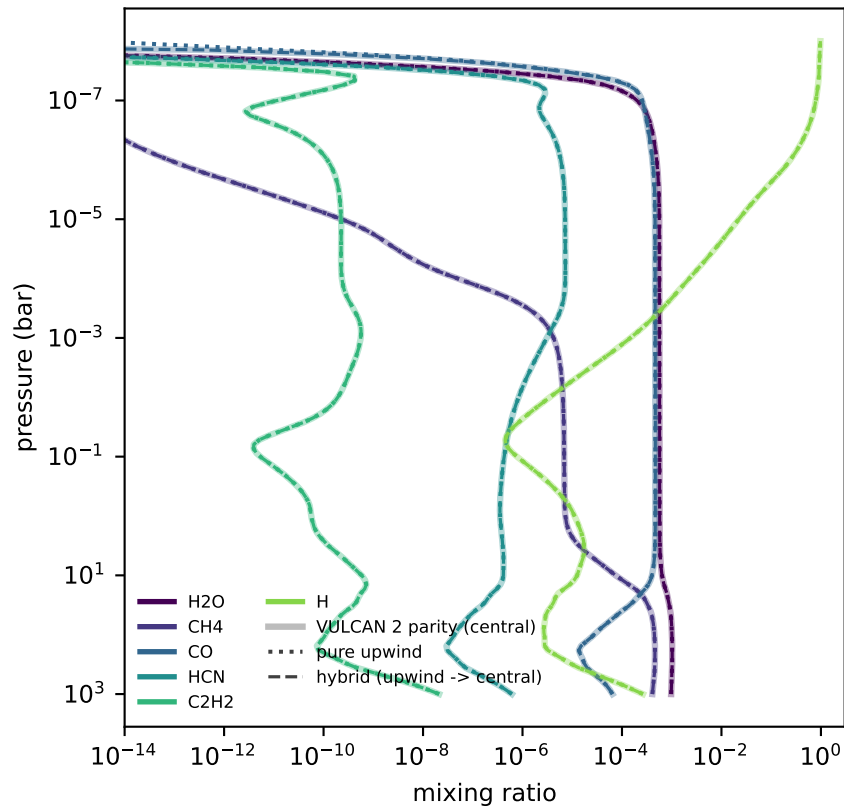
B final profiles: thick = central, dots = upwind, dash = hybrid
