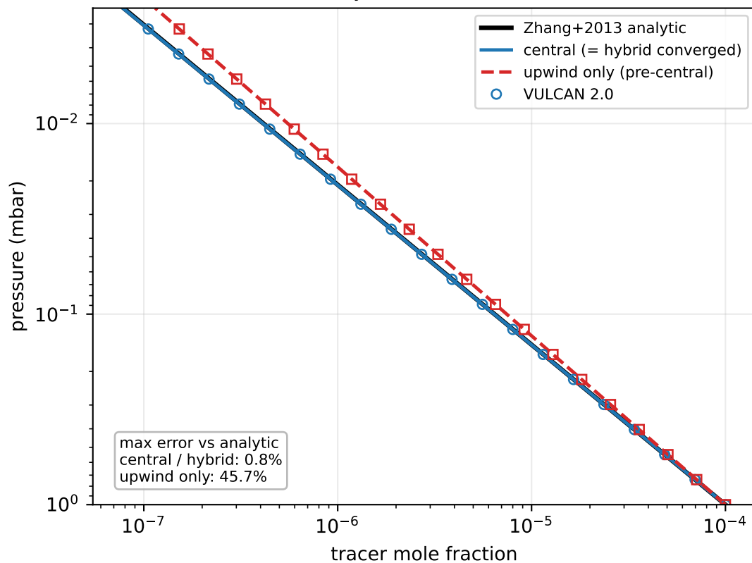
A. Accuracy (well resolved, n_z=120 )
