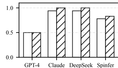
(5) free_bootmem-77
