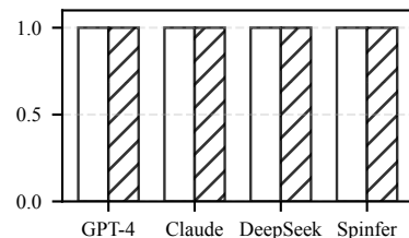
(12) tcf_block_get-61
