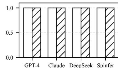
(9) snd_soc
