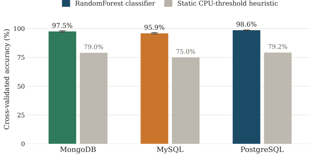
Fig. 1 RandomForest classifier accuracy versus the static CPU-threshold heuristic, by engine. Error bars show BCa 95% confidence intervals on the repeated 10 \times 5 -fold CV accuracy (Table 3); heuristic bars correspond to Table 4.
