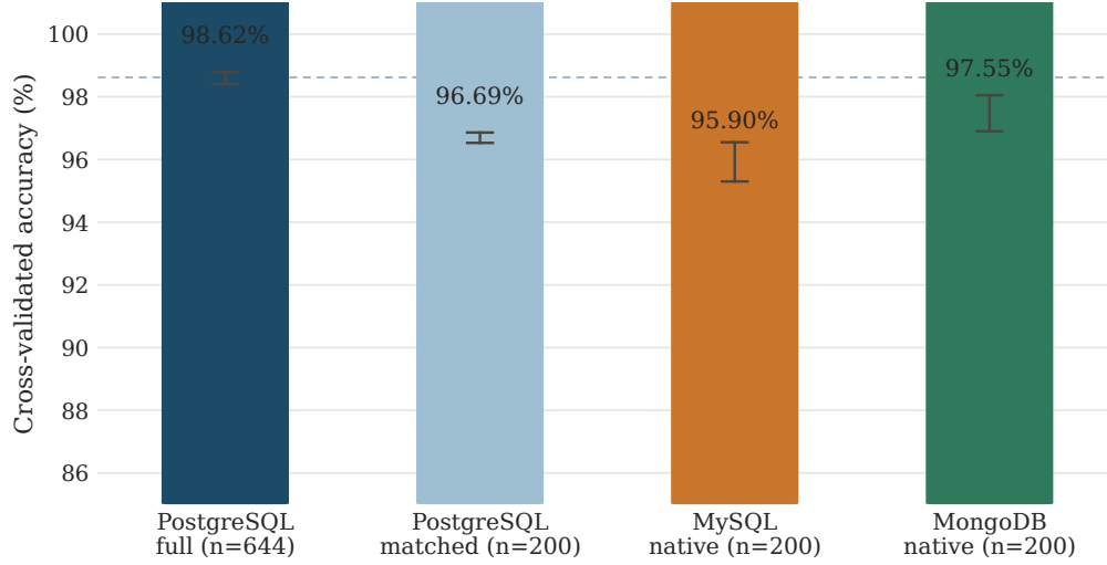
Fig. 2 Sample-size control: mean cross-validated accuracy for PostgreSQL at full size, PostgreSQL size-matched to n = 200 , and MySQL/MongoDB at their native n = 200 . Error bars show BCa 95% confidence intervals (Table 6); the dashed line marks full-size PostgreSQL accuracy for reference.
