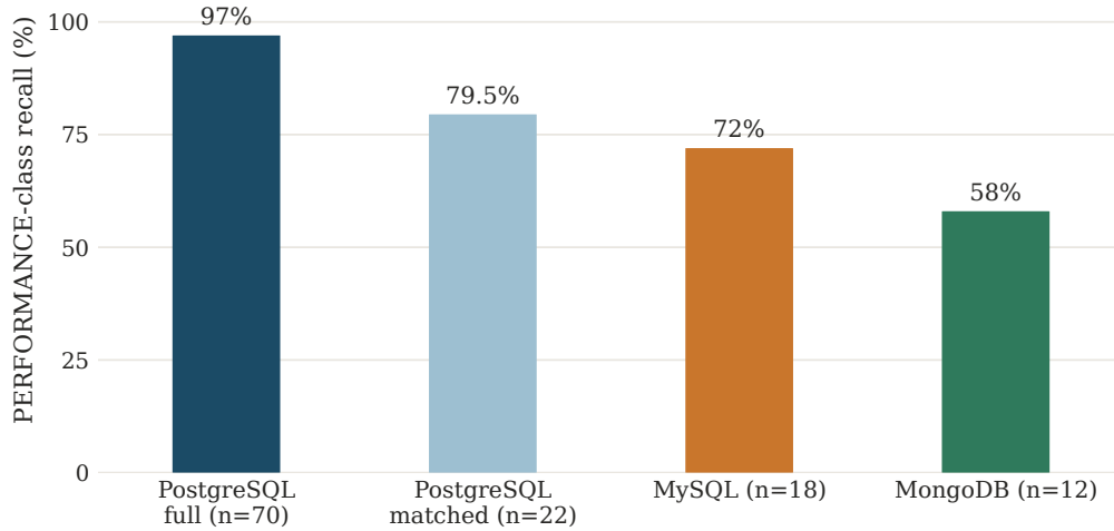
Fig. 3 PERFORMANCE-class recall as a function of the number of PERFORMANCE training examples available, across the four conditions in Table 7.
