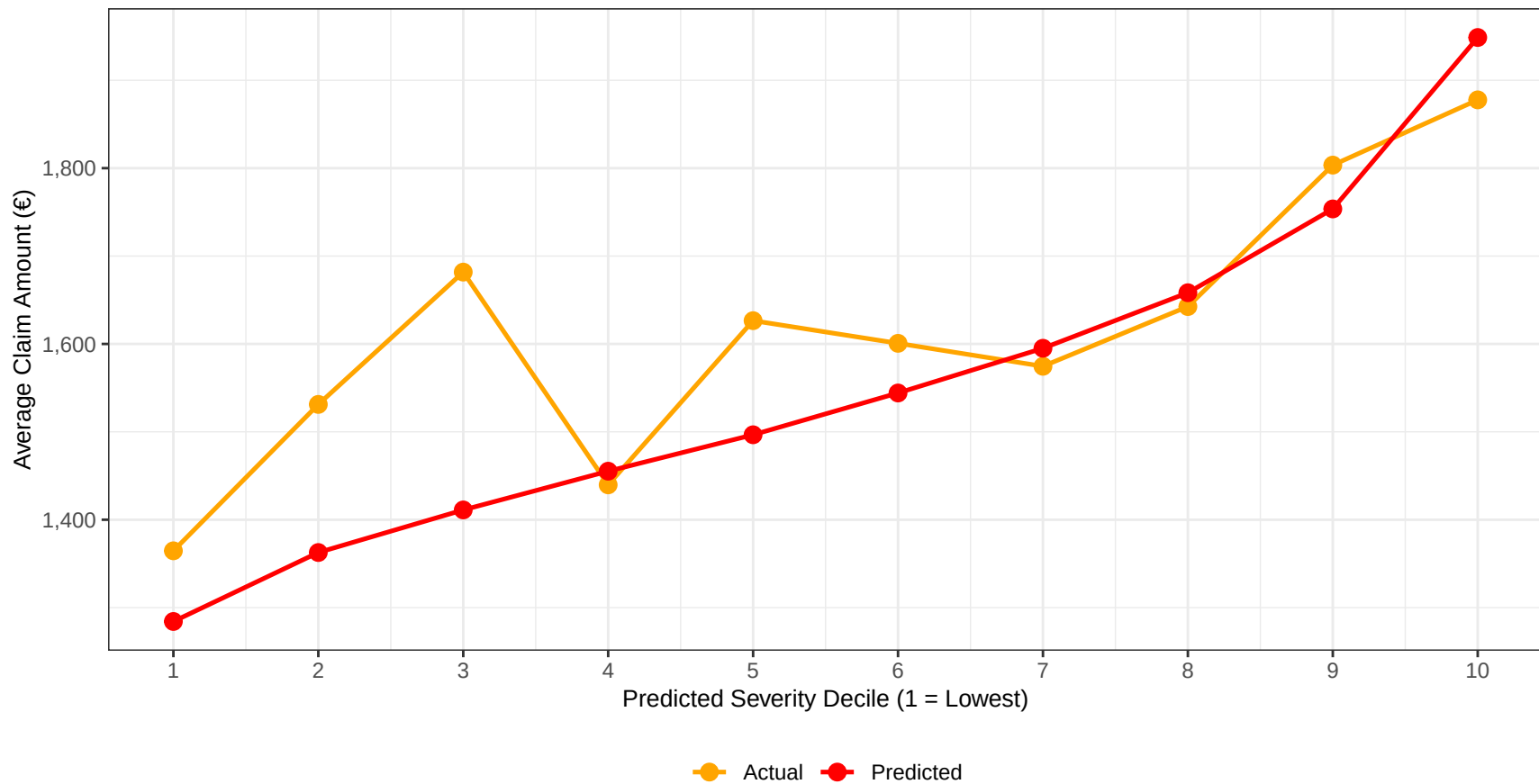
Severity Model: Decile Lift Chart (Test Set)
