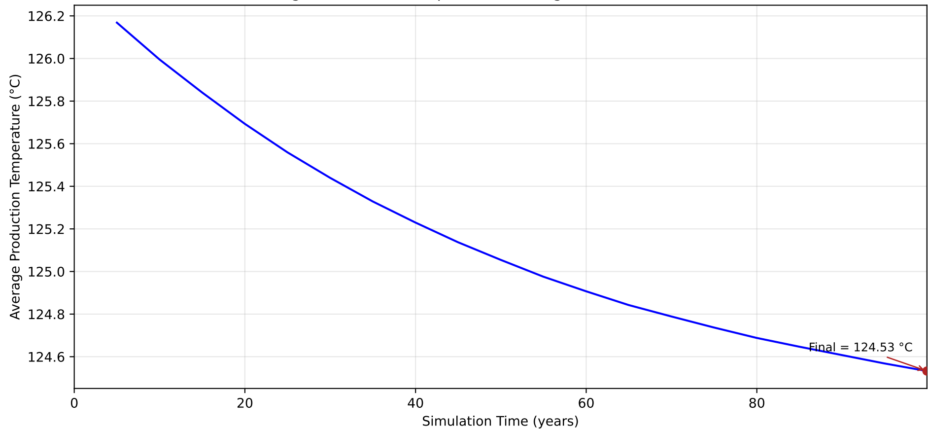
Average Production Temperature During the 100-Year Simulation
