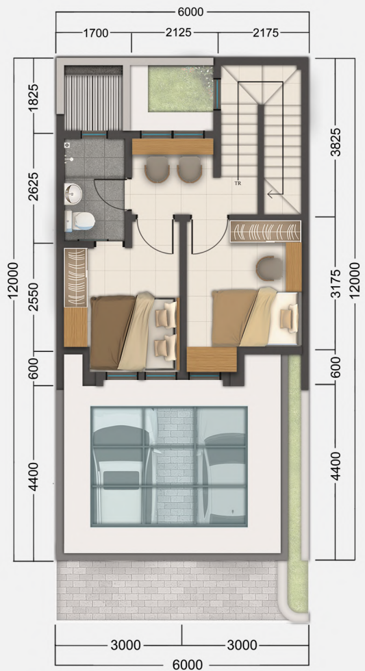
Second Floor
