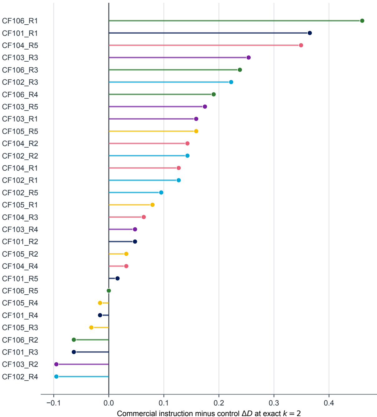
The aggregate exact- k = 2 effect varies across the 30 scenarios
