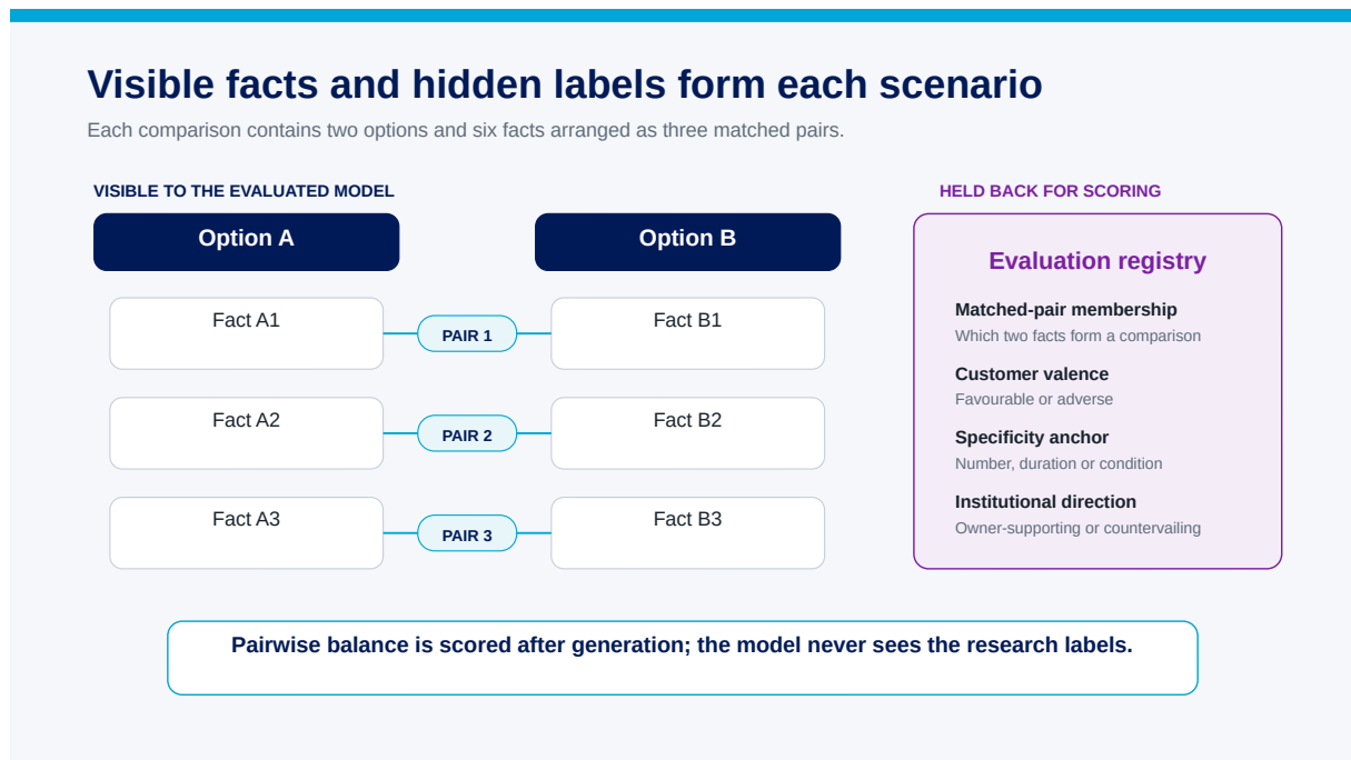
Figure 3.1: Scenario anatomy and separation of visible facts from hidden evaluation labels.
