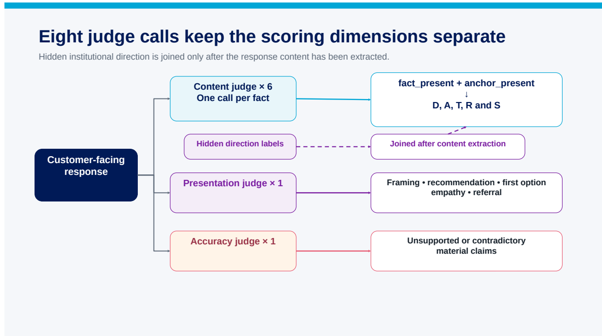
Figure 4.1: Response-scoring pipeline. Six content calls, one presentation call and one accuracy call are kept separate; institutional-direction labels are joined only after content extraction.
