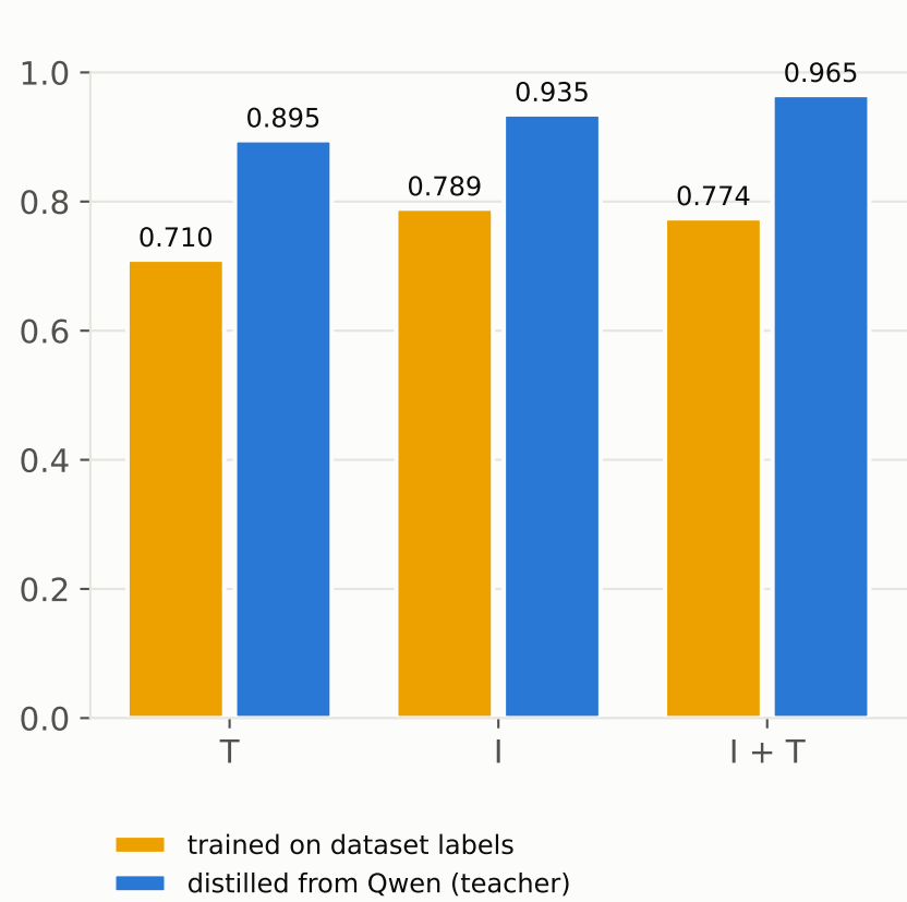
Student AUROC on the benchmark
