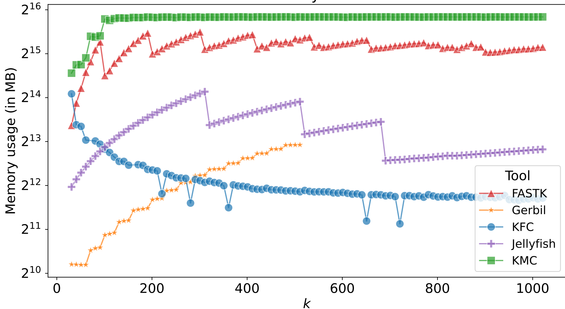
Memory vs k
