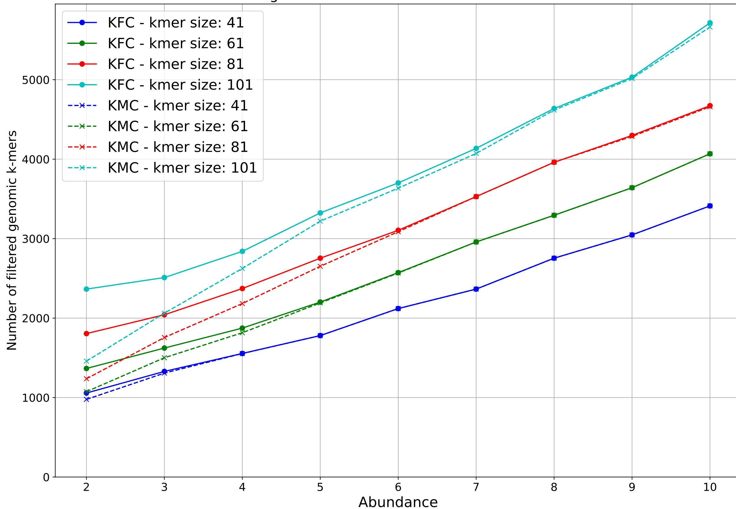
Number of filtered genomic k-mers vs abundance for different k-mer sizes
