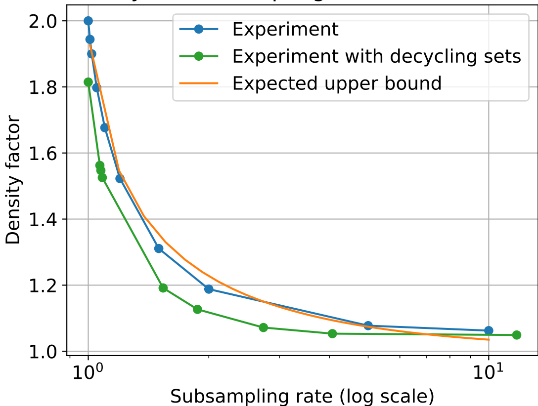
Density vs Subsampling rate ( k=31, m=15 )
