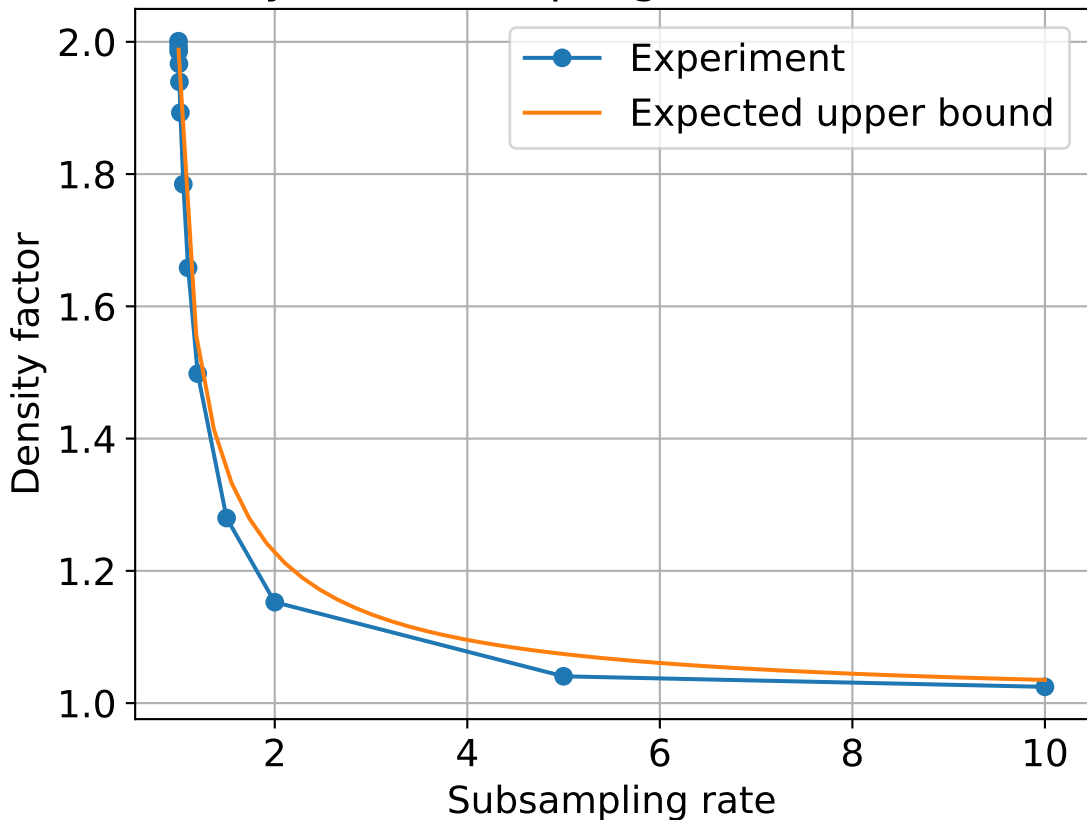
Density vs Subsampling rate ( k=63, m=15 )
