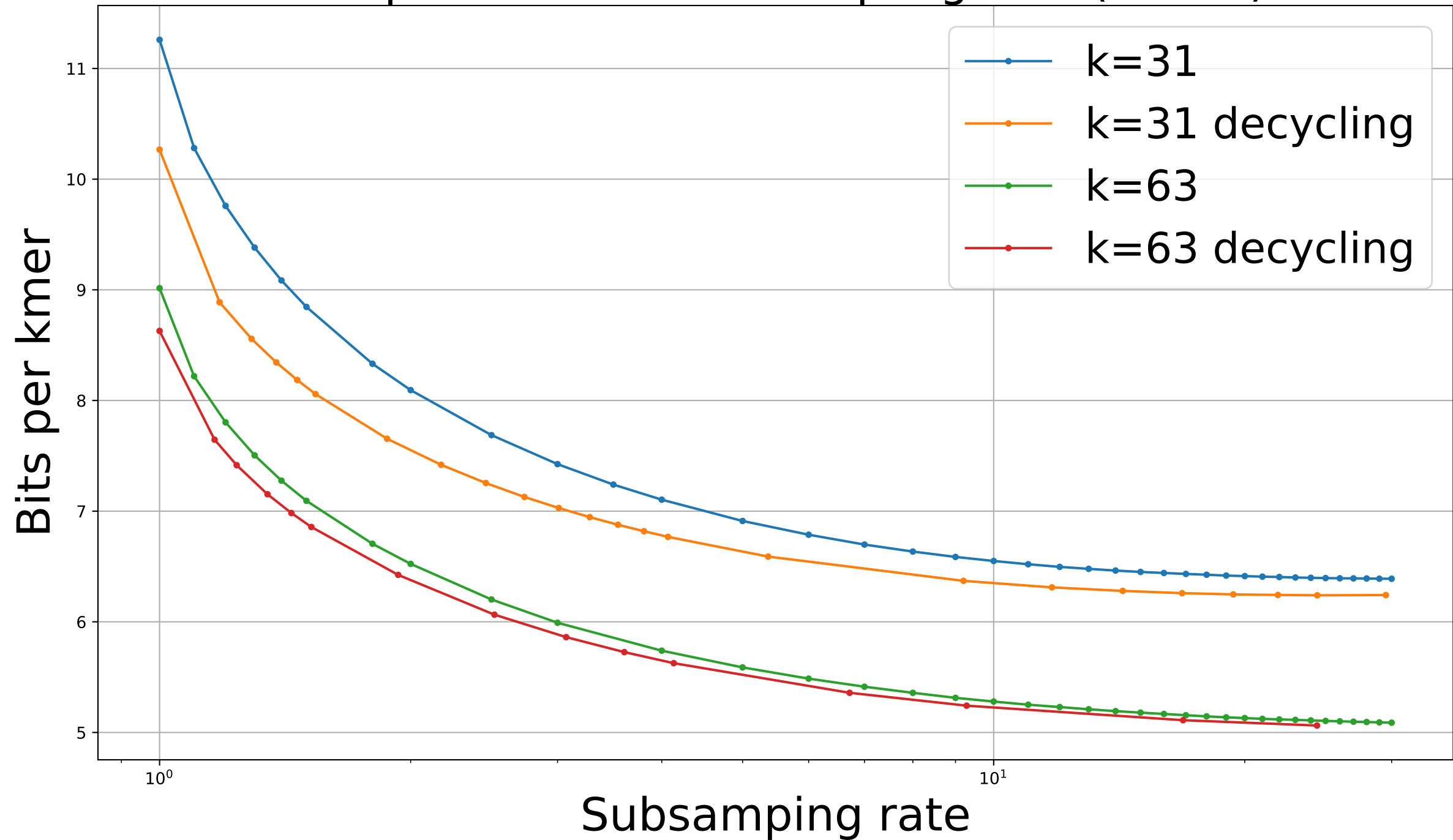
Bits per kmer vs Subsampling rate (m=15)
