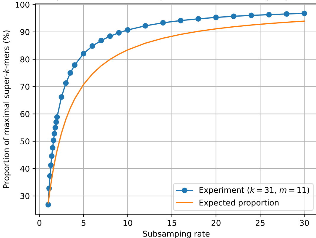
Proportion of maximal super- k -mers vs Subsampling rate
