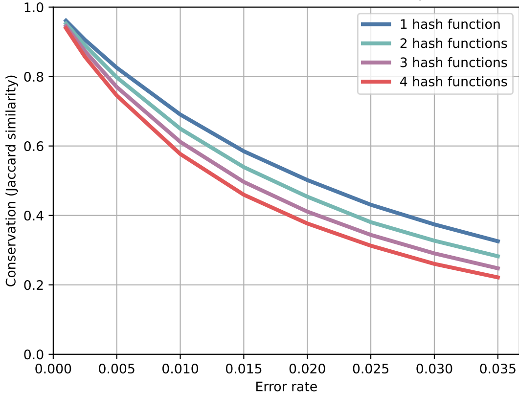
Conservation of multimiminizers on random text ( m = 21 , w = 15 )
