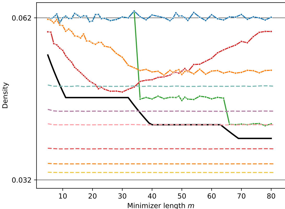
Minimizer density on random text ( w = 31 )
