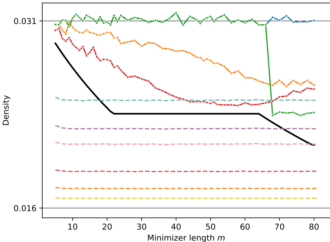
Minimizer density on random text ( w = 63 )
