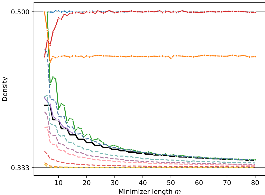
Minimizer density on random text ( w = 3 )
