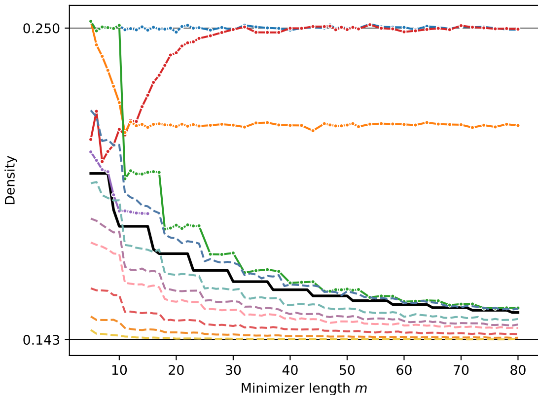
Minimizer density on random text ( w = 7 )
