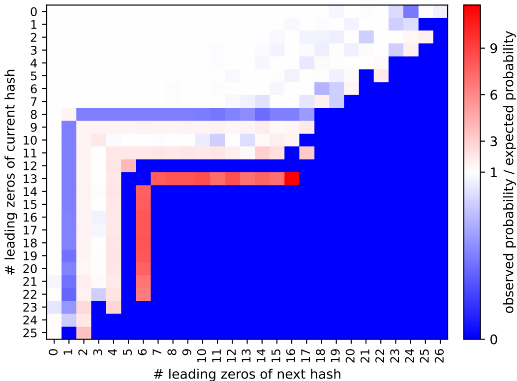
Bias of leading-zero transition (vs geometric dist.) R = 7, k = 31
