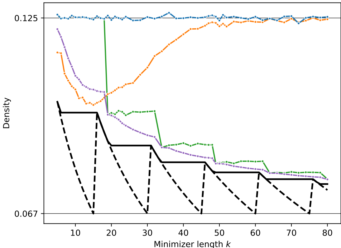
Minimizer density on a random sequence ( w = 15 )
