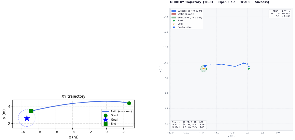
(a) UHRC under nominal dynamics (100% model certainty). (b) UHRC under perturbed dynamics (80% model certainty).
