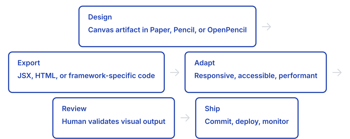
The five-stage deploy pipeline from design artifact to production with agent and human roles
