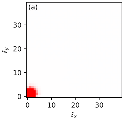
Trivial ( C = 0 )
