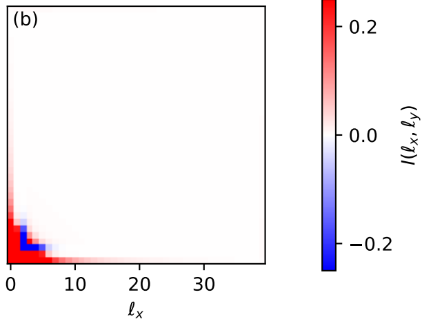
Topological ( C = 1 )
