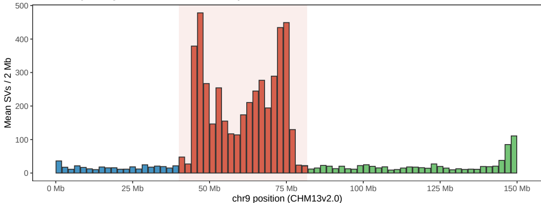
SV density along chromosome 9, all samples
