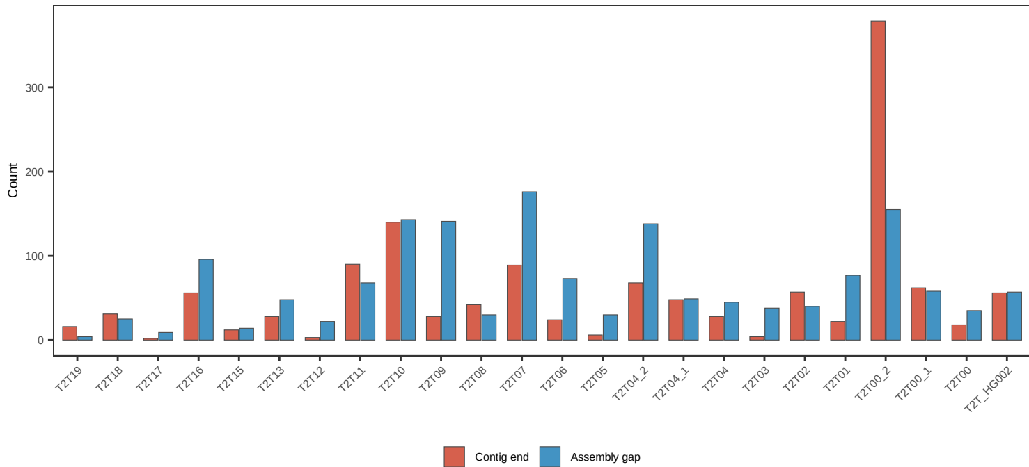
Contig ends and gaps in multicopy gene loci per sample
