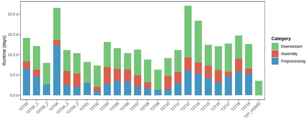
Pipeline runtimes on a single node, 72 threads, 2GPU
