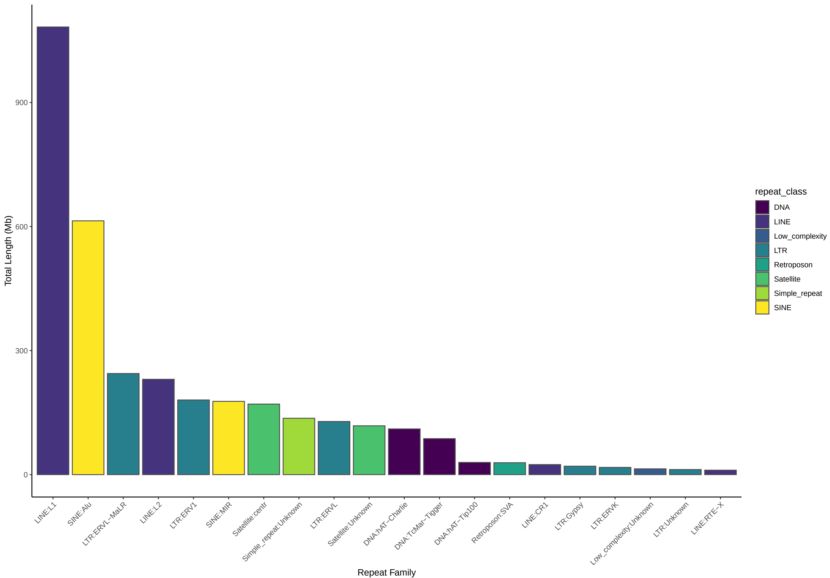
Top 20 Repeat Families
