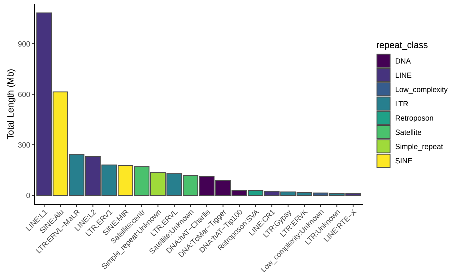
Top 20 Repeat Families
