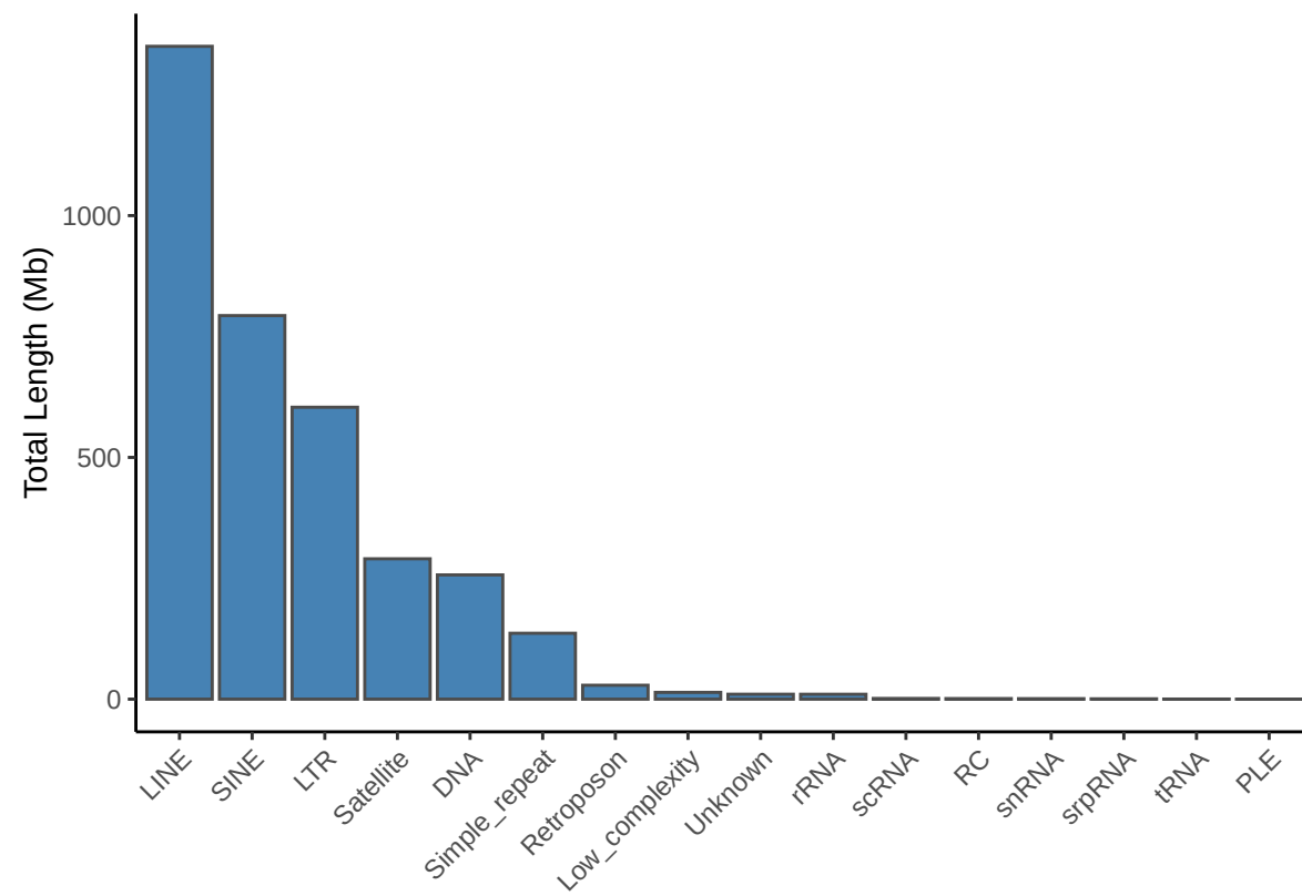
Distribution of Repeat Classes
