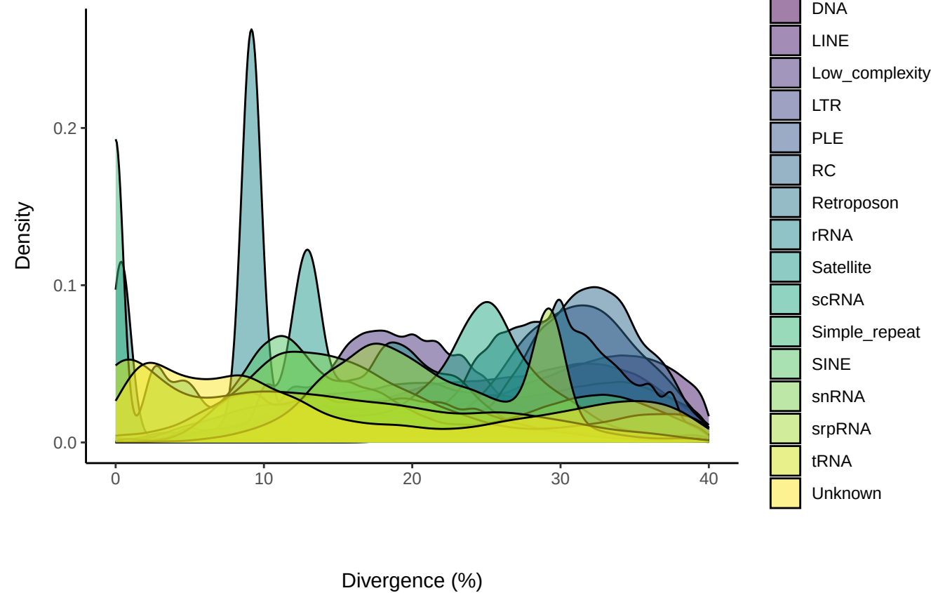
Divergence Distribution by Repeat Class
