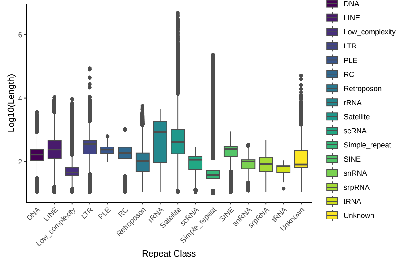
Length Distribution by Repeat Class
