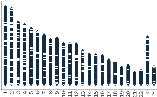
Nucflag
