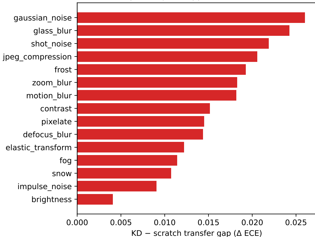
Knowledge distillation's calibration-transfer penalty by corruption type (CIFAR-10-C)
