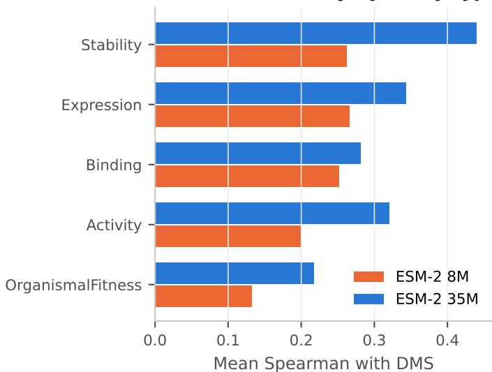
Zero-shot accuracy by assay type
