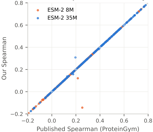
Our scorer reproduces ProteinGym
