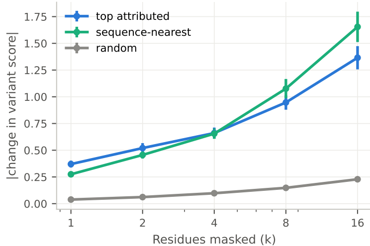
Deletion test, ESM-2 35M
