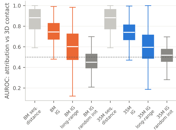
Attributions find 3D neighbours
