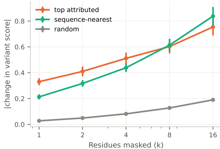
Deletion test, ESM-2 8M
