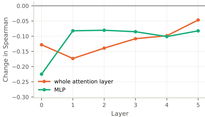
ESM-2 8M: layer ablations
