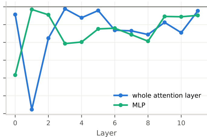
ESM-2 35M: layer ablations
