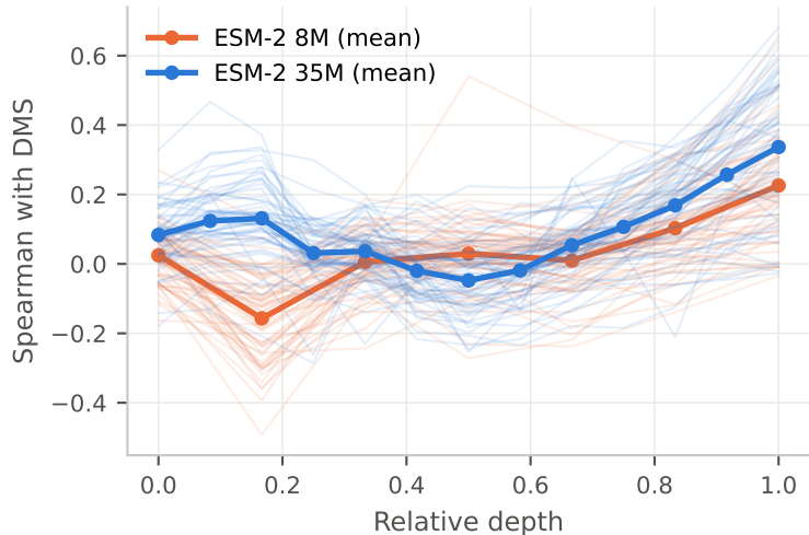
Logit lens: when the variant signal appears
