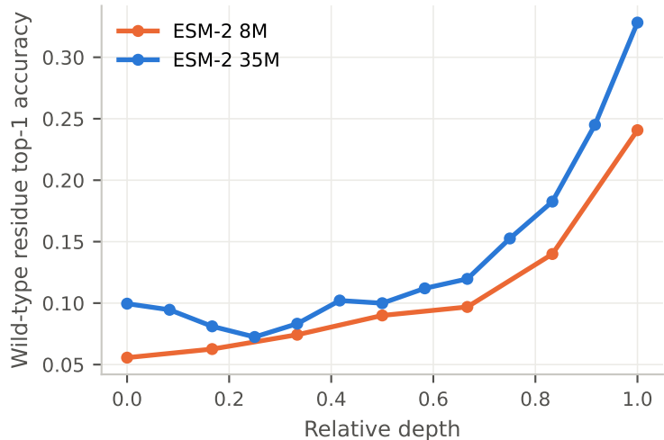
Logit lens: recovering the masked residue
