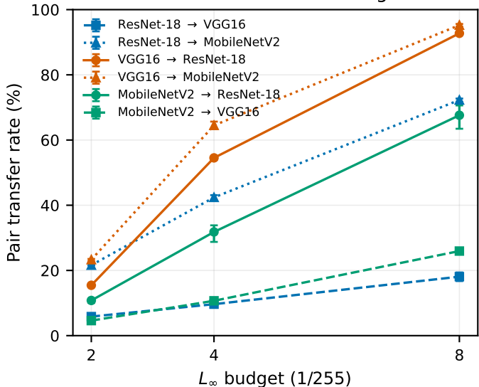
PGD transfer versus budget
