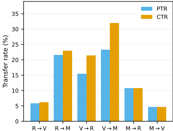
Conditioning at 2/255 PGD
