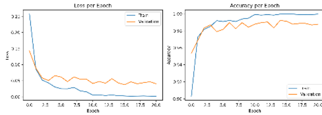
(a) Training and validation loss and accuracy.
