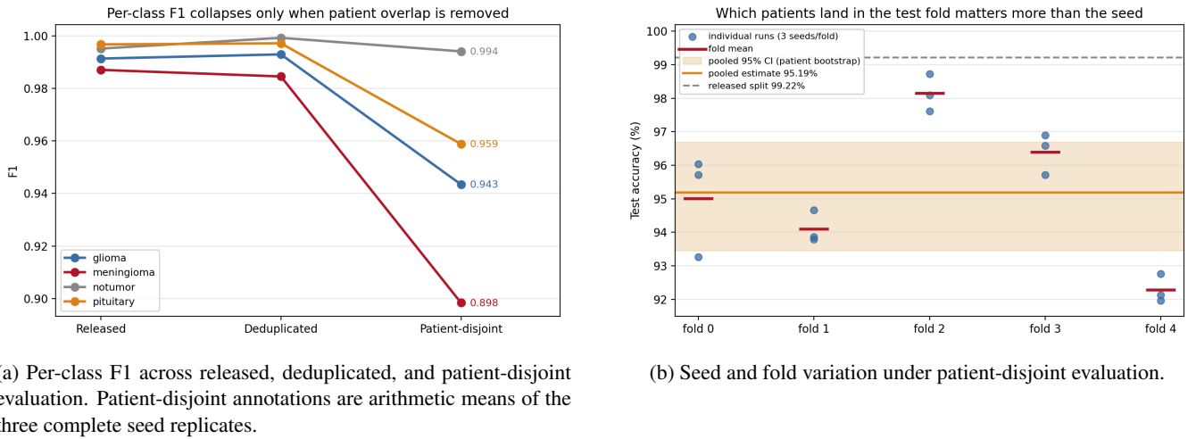
Figure 3: Performance heterogeneity becomes visible only after patient grouping.
