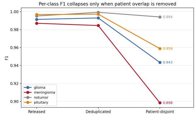
Figure 7: Per-class F1 across the three splits. Deduplication leaves every class essentially unchanged; removing patient overlap separates them, and meningioma falls furthest. Generated by make_cv_figures.py .
