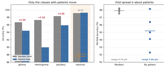
Figure 9: The matched random-split control. Left: per-class accuracy under random and patient-grouped folds, with the paired difference above each pair. The three classes with patient identity all move; notumor , which has none, does not. Right: per-fold accuracy in each arm. Folds that ignore patients are interchangeable, folds that respect them are not.
