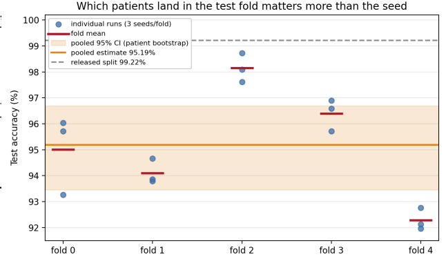
Figure 10: Per-fold accuracy against the pooled cross-validated estimate. Within-fold scatter is seed variance; between-fold scatter is partition variance, and it is the larger of the two. A single patient-disjoint holdout could have landed anywhere in this range.
