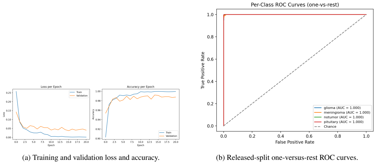
Figure S2: Released-split training dynamics and ranking performance. These results are measured under patient leakage.
