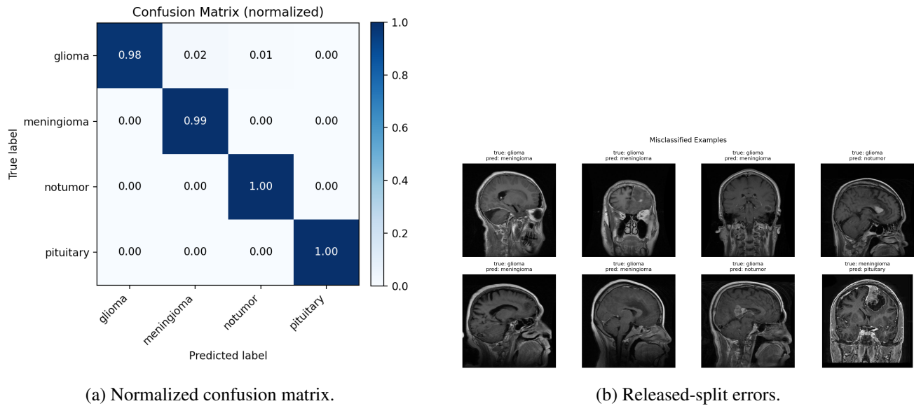
Figure S3: Released-split error analysis, provided for reproducibility rather than as evidence of generalization.
