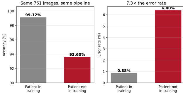
Figure 12: The same 761 test images scored by models that did and did not train on the patient, with everything else held constant. Accuracy differs by 5.5 points; the error rate differs by a factor of 7.3.
