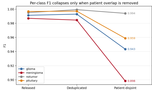
Figure 11: Per-class F1 across the three splits. Deduplication leaves every class essentially unchanged; removing patient overlap separates them, and meningioma falls furthest. Generated by make_cv_figures.py .
