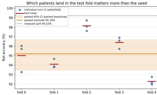
Figure 13: Per-fold accuracy against the pooled cross-validated estimate. Within-fold scatter is seed variance; between-fold scatter is partition variance, and it is the larger of the two. A single patient-disjoint holdout could have landed anywhere in this range.
