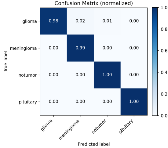
Figure 14: Test-set confusion matrix, normalized by true class.
