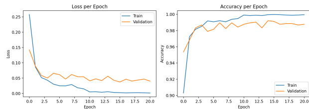
Figure 13: Training and validation loss and accuracy per epoch. Training loss approaches zero while validation loss plateaus, which is what triggers early stopping at epoch 21.
