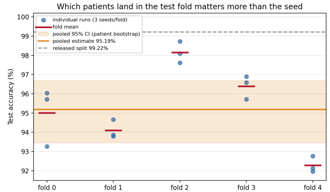
Figure 9: Per-fold accuracy against the pooled cross-validated estimate. Within-fold scatter is seed variance; between-fold scatter is partition variance, and it is the larger of the two. A single patient-disjoint holdout could have landed anywhere in this range.
