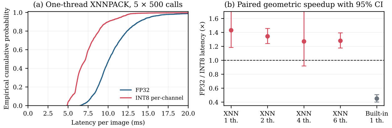
Fig. 1. Latency audit. (a) Pooled one-thread XNNPACK empirical CDFs contain 2,500 observations per precision from five process restarts. (b) Points are paired geometric-mean FP32/INT8 speedups; bars are log- t 95% intervals across five matched process means. Values above one favor INT8.
